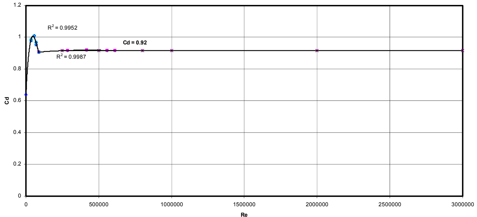
BFM Cd versus Re All Contoured Plates Tested To-Date
